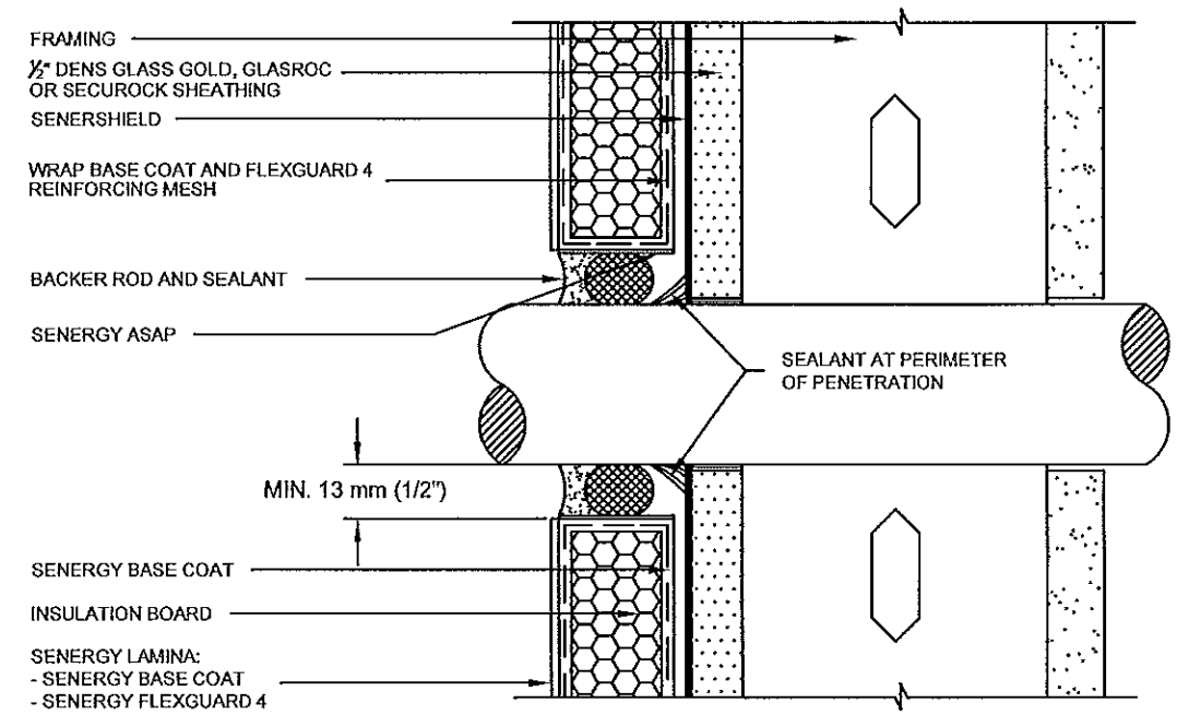
PIPE PENETRATION
